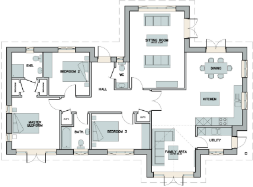
FLOOR PLAN EXTERNAL FLOOR AREA - 161.83M 2 0 5 10M
